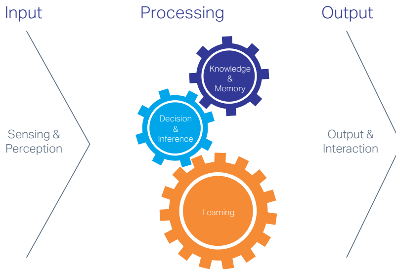
Figure 1. Human intelligence
