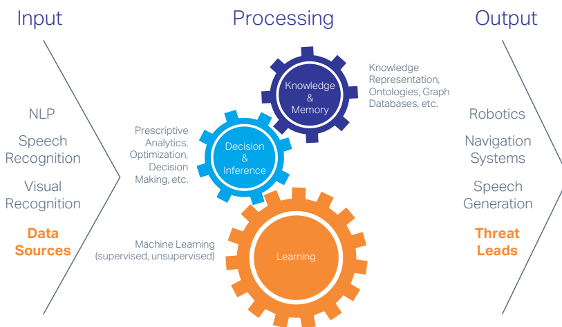
Figure 2. Artificial intelligence
