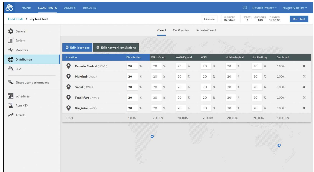
Figure 3. Edit locations in LoadRunner Cloud
