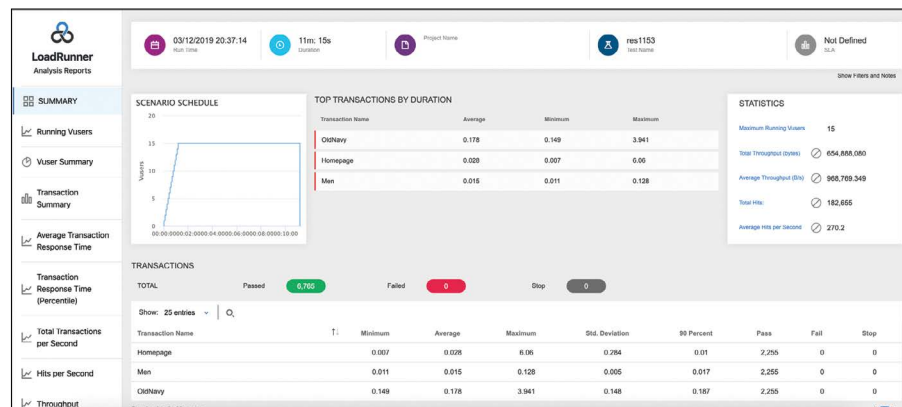
Figure 7. LoadRunner Professional Analysis Summary
