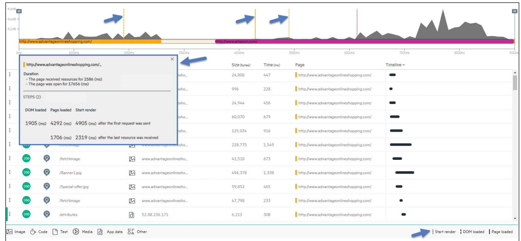
Figure 6. Client-side Breakdown Report
