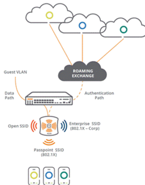
Aruba AirPass System Architecture
