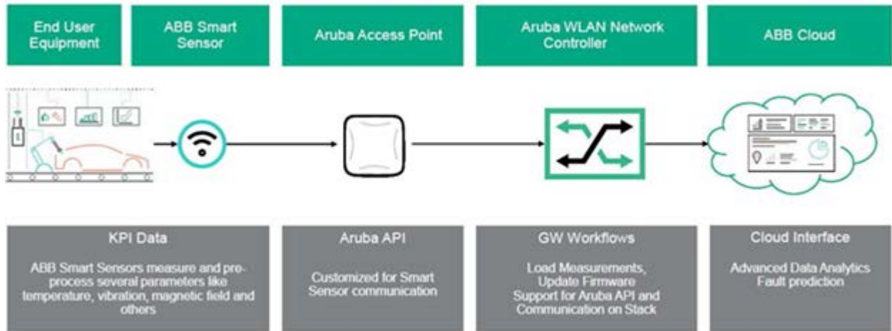
Aruba and ABB Integration Overview
