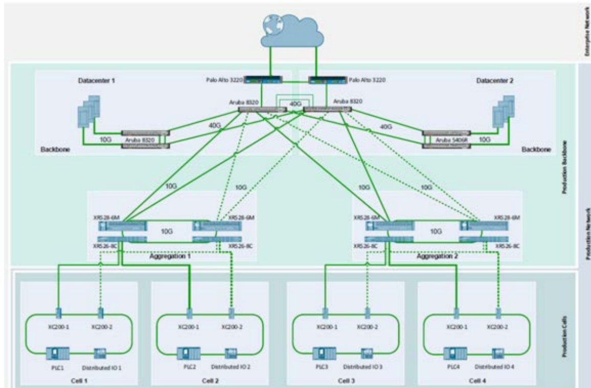
Typical Joint Deployment Scenario
