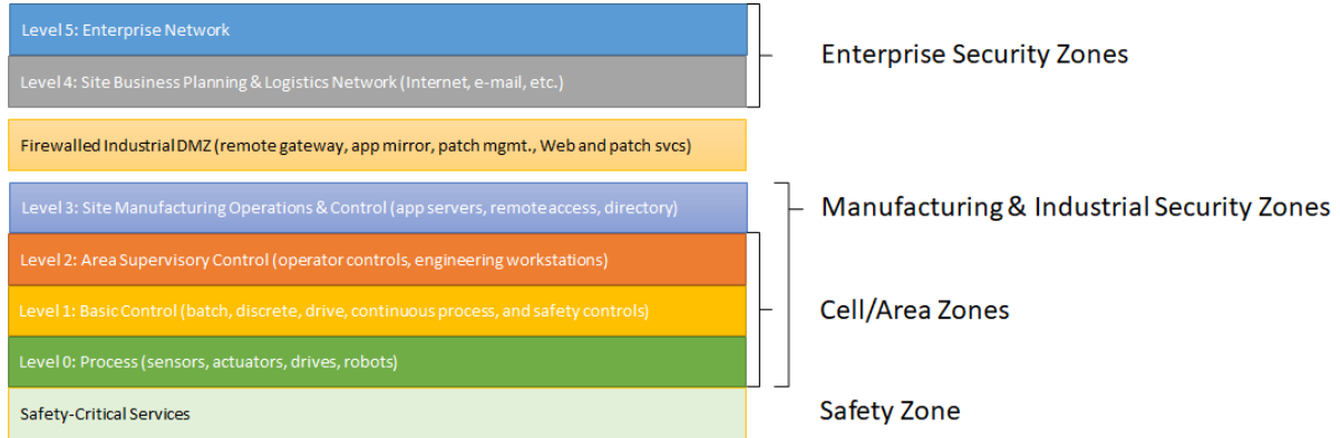
Classic Purdue Model
