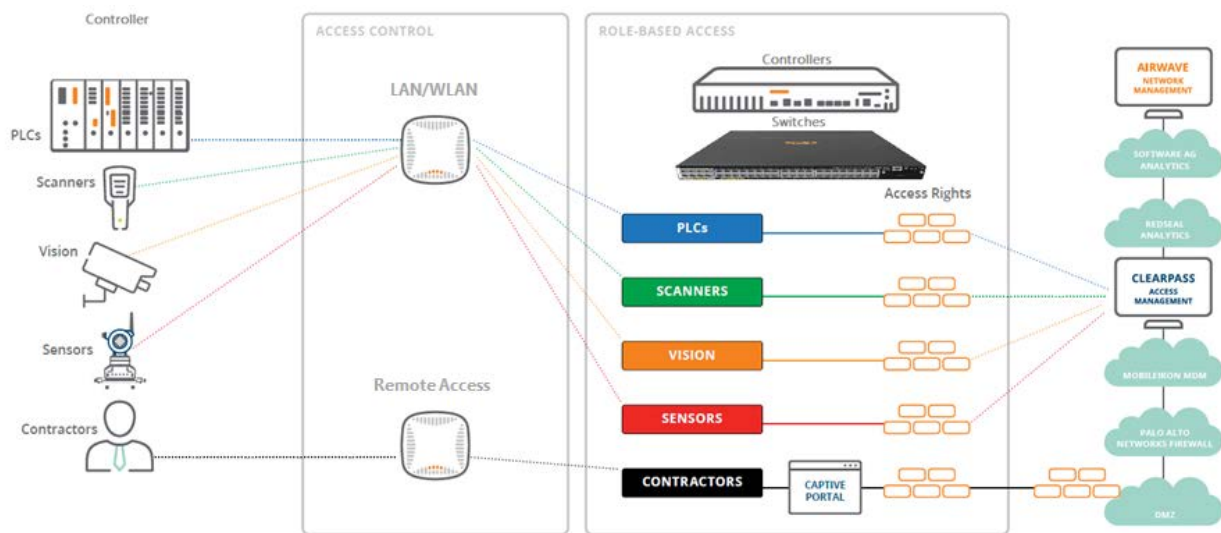
Using Aruba's AI And Policy Enforcement Firewall Services To Connect And Protect Profinet IO
