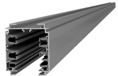
Starline Track Busway 250 Amp Housing
