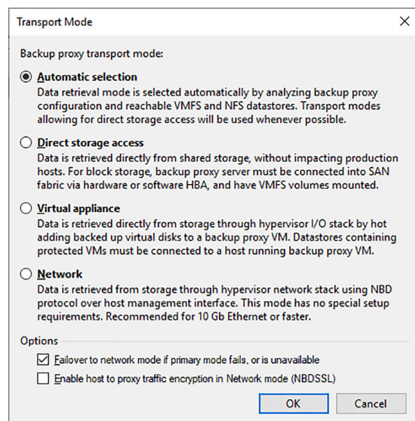
Figure 1: Transport mode options
