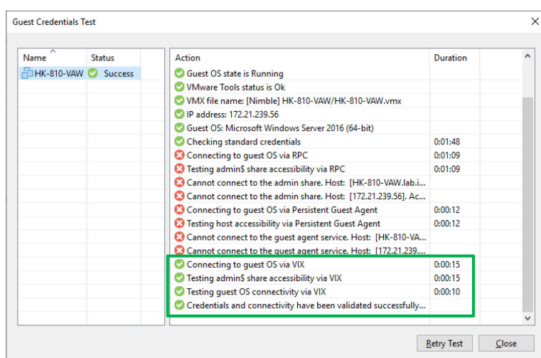
Figure 7: Guest credentials test via VIX API
