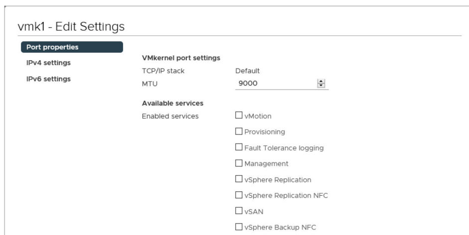
Figure 3: No services enabled for VMkernel port
