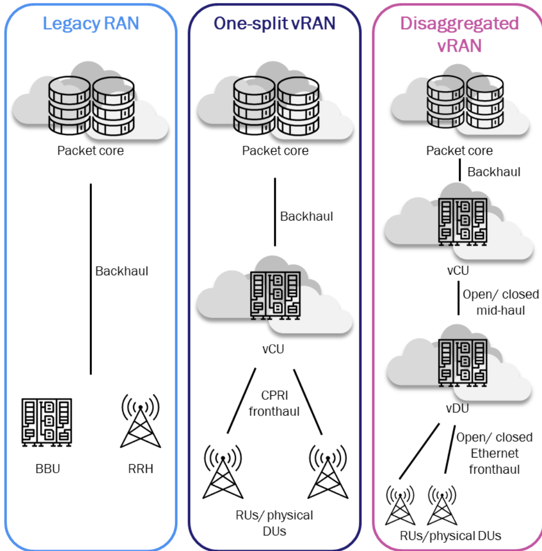
Figure 2.1: Overview of the architecture for the legacy RAN, the one-split vRAN and the disaggregated vRAN
