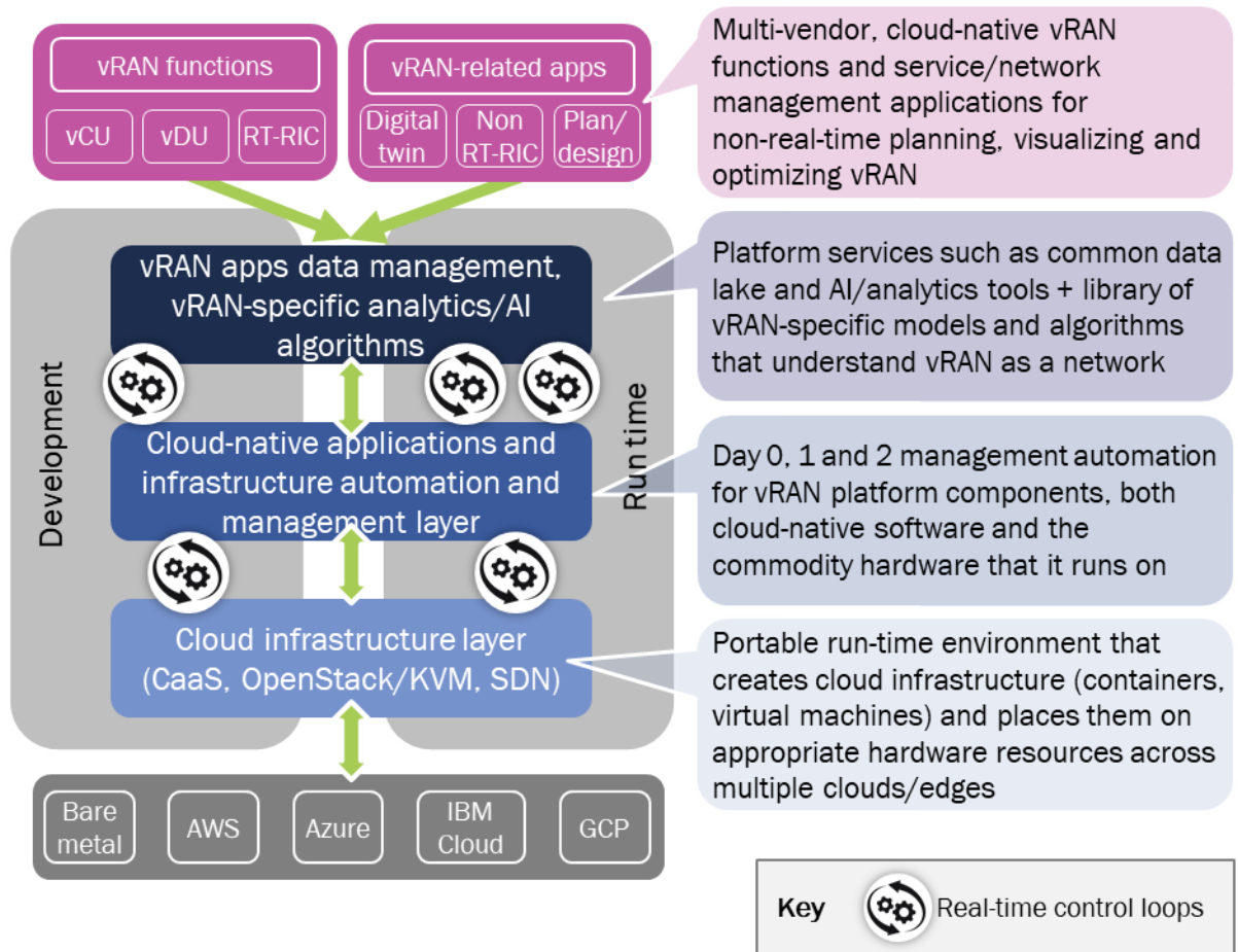
Figure 3.2: A vRAN architected as a platform
