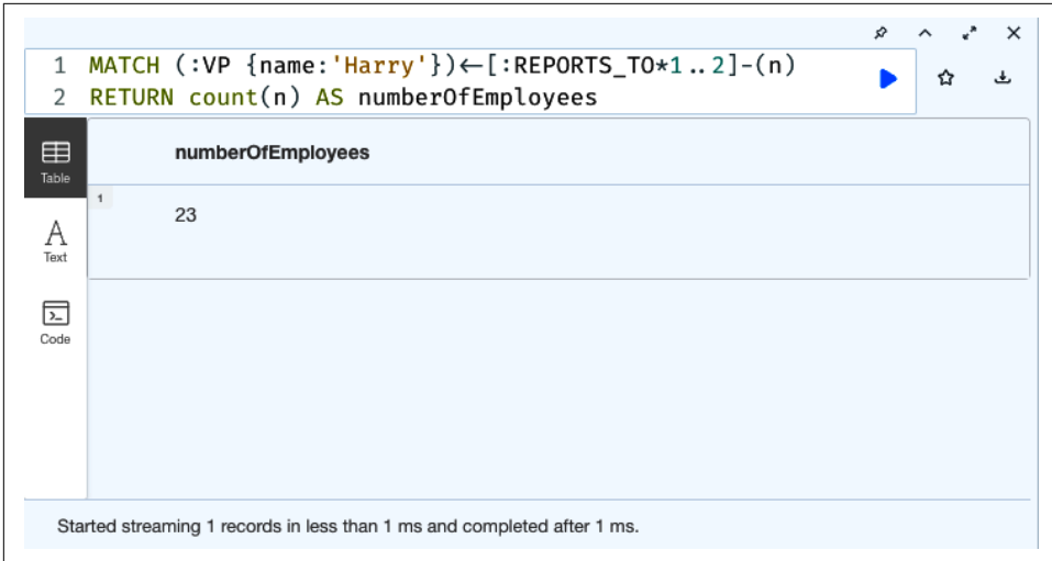
Figure 10-9. Aggregating the number of employees in a particular department
