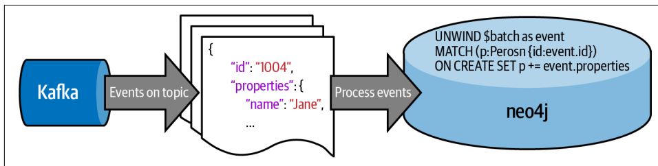
Figure 5-9. Receiving messages from Kafka and using Cypher MERGE to insert data into the knowledge graph
