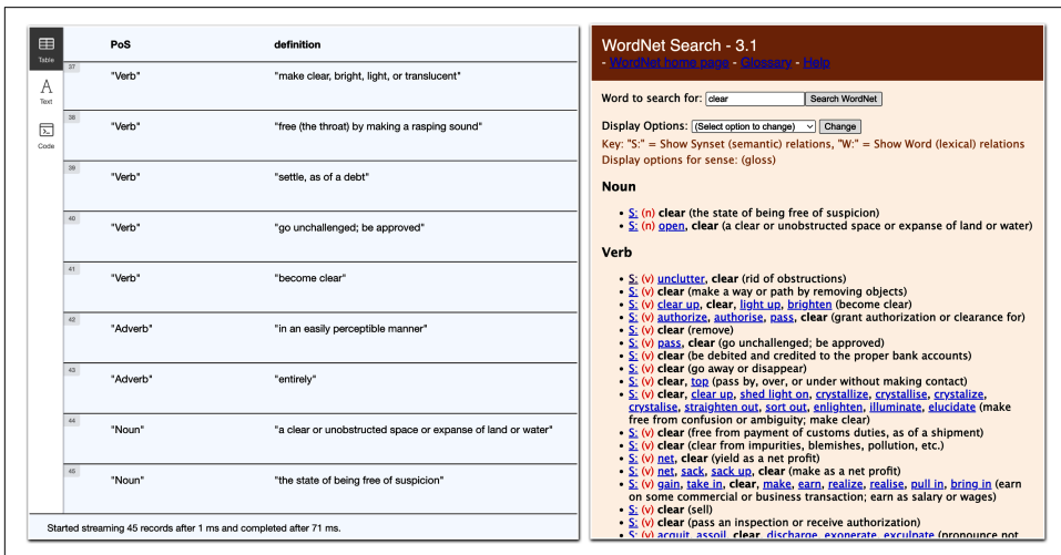
Figure 13-5. WordNet results for the meaning of clear are the same in the Neo4j Browser (left) and WordNet's web interface (right)
