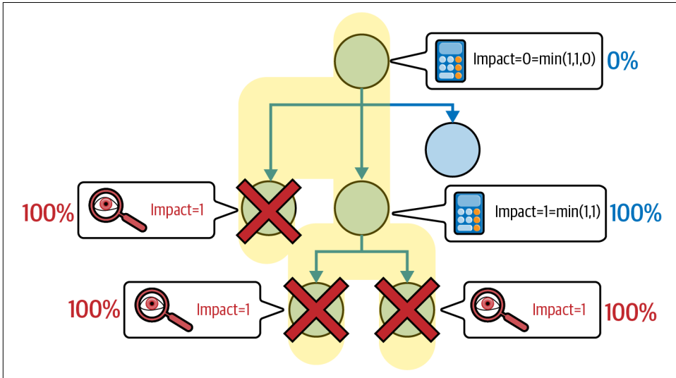
Figure 11-5. Impact propagation in aggregate multidependencies
