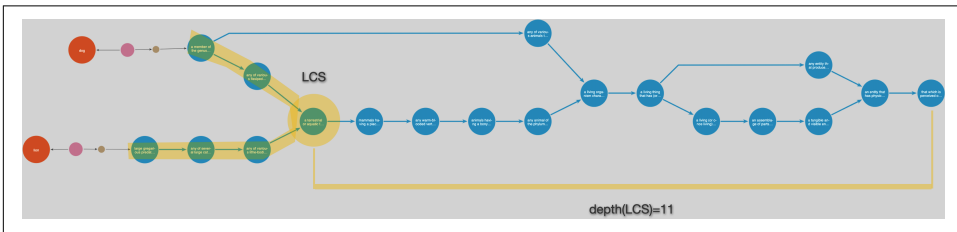
Figure 13-13. The Wu-Palmer distance
