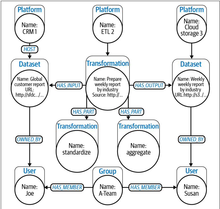
Figure 3-3. A graph describing a simple data pipeline
