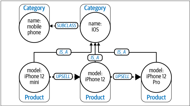
Figure 2-6. An ontology showing upgrade paths (upsell opportunities) for products in the catalog
