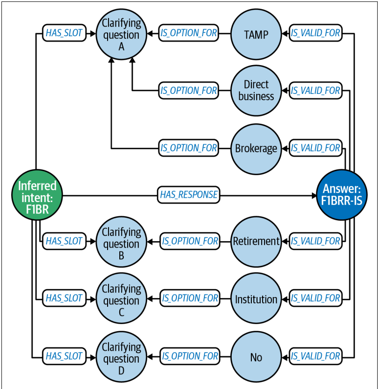
Figure 5-7. Representation of the LPL Financial subgraph used for a financial chatbot
