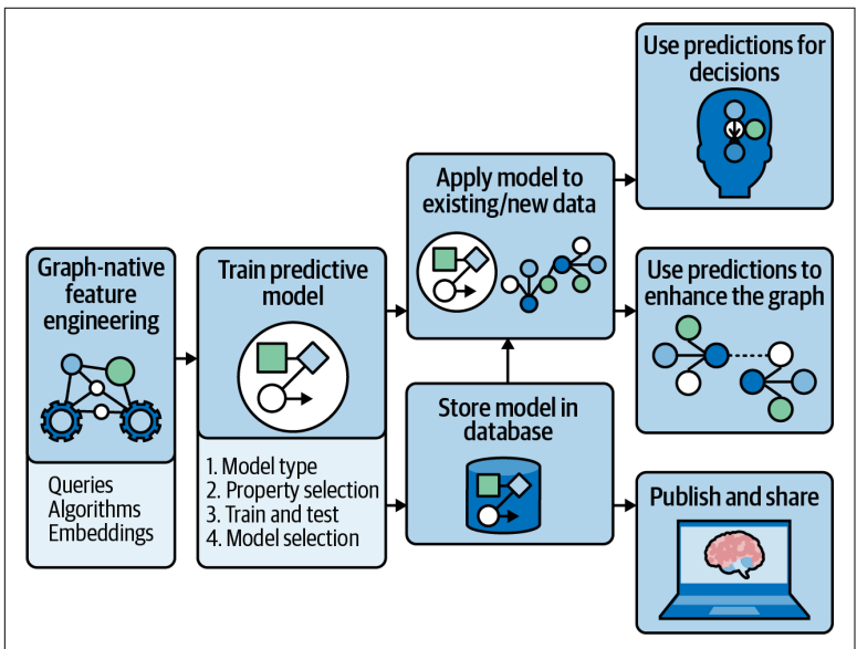
Figure 4-4. A closed-loop graph ML workflow
