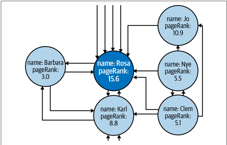
Figure 4-3. Node importance via the PageRank algorithm
