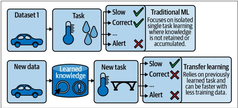
Figure 5-2. Example of traditional ML versus transfer learning for a semiautonomous vehicle
