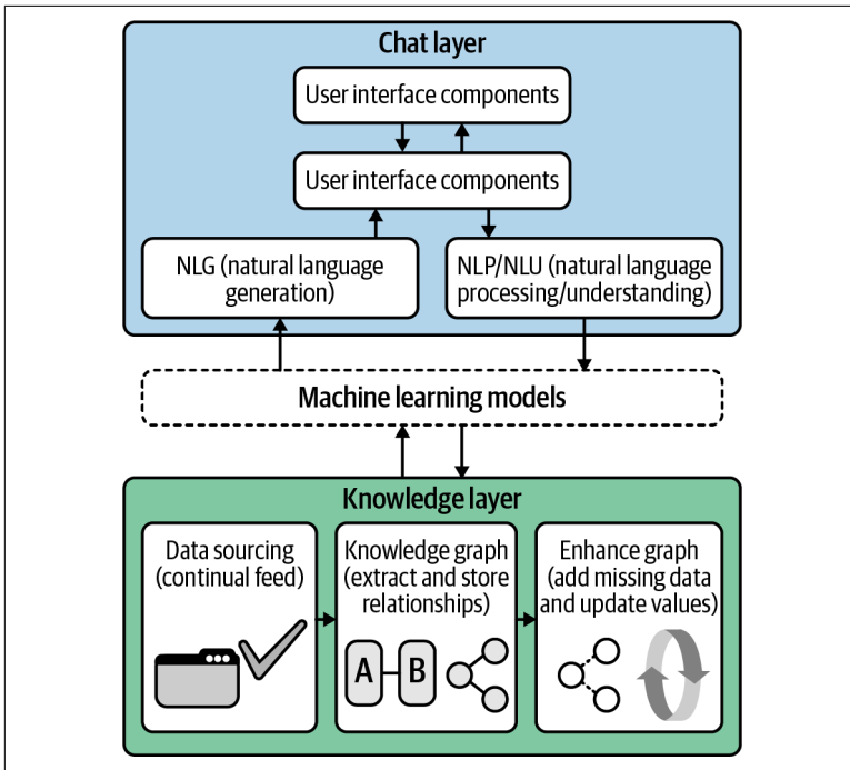
Figure 5-6. Chatbot system architecture proposed by researchers 3
