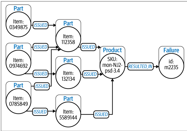
Figure 4-5. Illustrative example of a simple graph similar to Boston Scientific's data model
