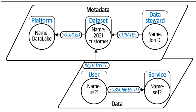
Figure 3-1. Relationships connect the data and metadata layers
