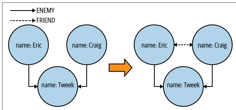
Figure 4-2. Making friends with the enemy of my enemy.
