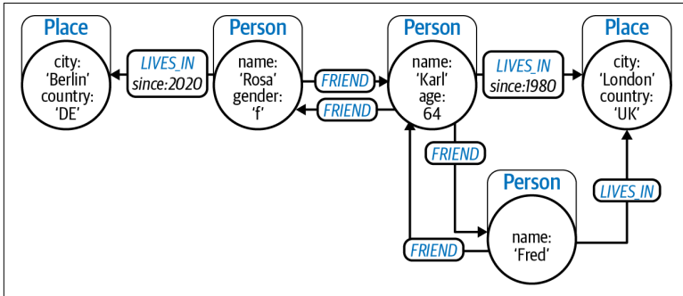
Figure 1-3. A graph representing people, their friendships, and their locations
