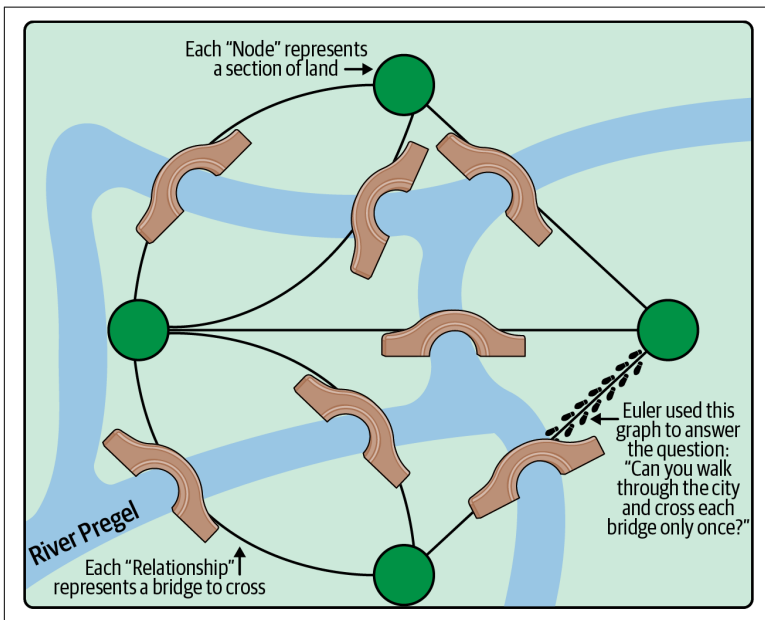
Figure 1-2. A graphical representation of Königsberg and its seven bridges crossing the River Pregel
