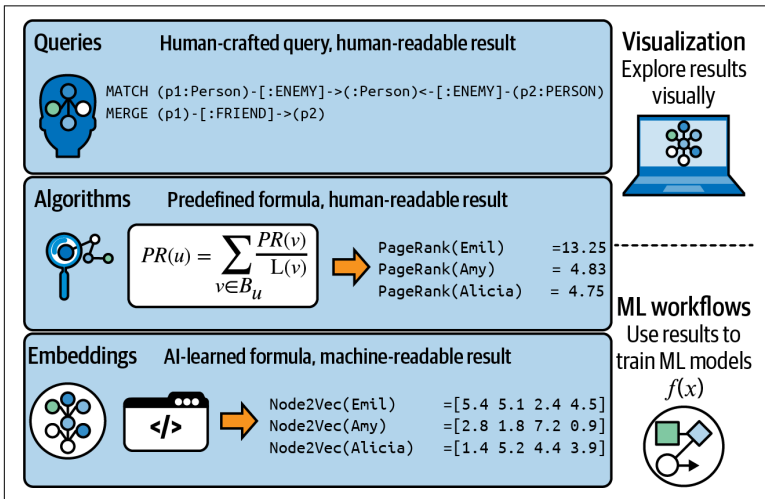
Figure 4-1. Unique capabilities combined in a decisioning knowledge graph
