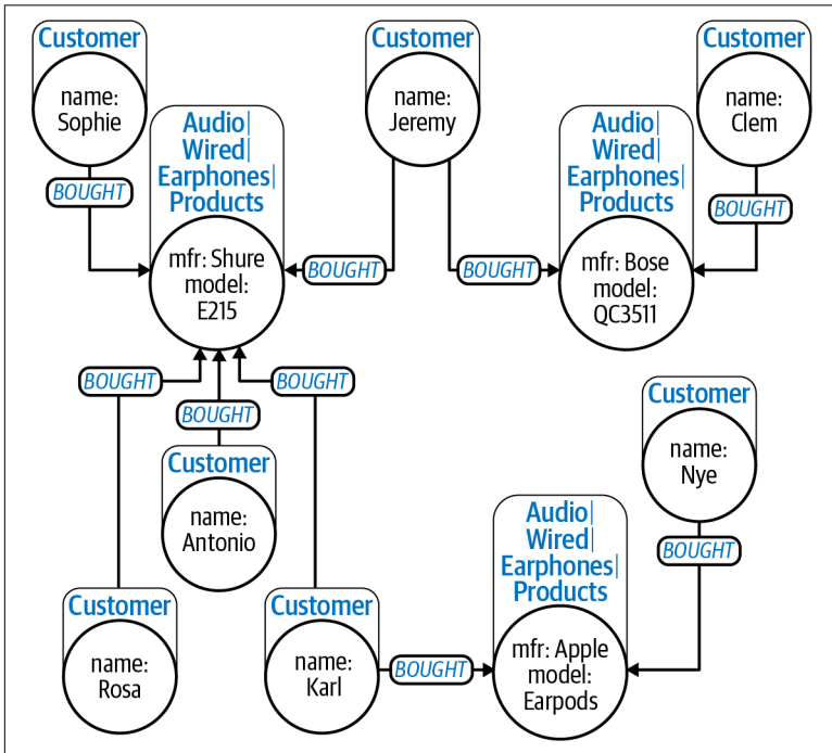
Figure 2-2. A snapshot of customers and their purchases as a property graph
