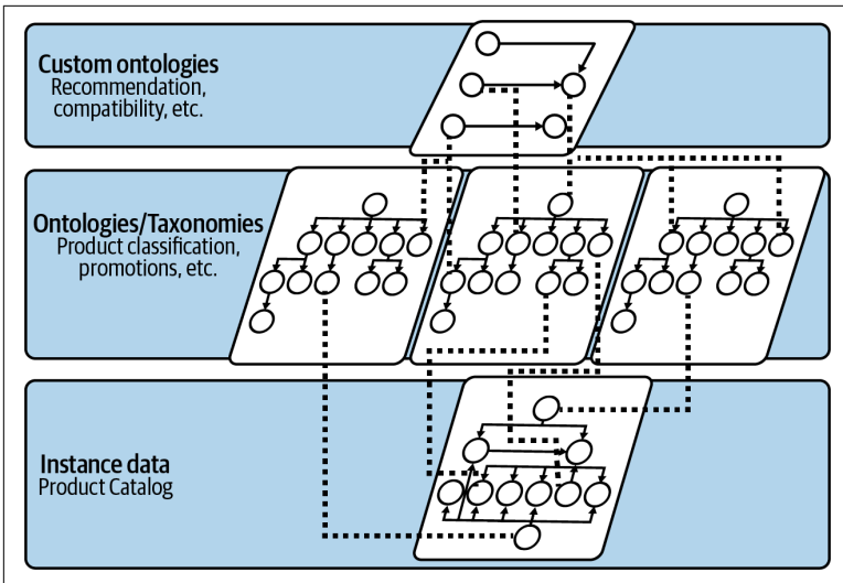
Figure 2-7. A sophisticated layering of ontologies and taxonomies over the same data set
