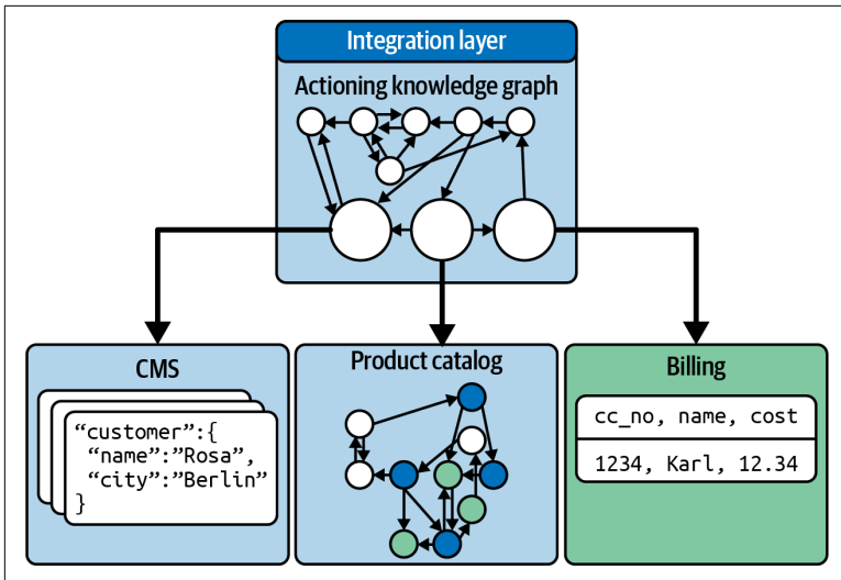
Figure 3-2. An actioning knowledge graph supported by a data fabric
