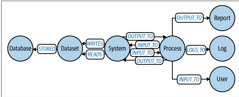
Figure 5-4. Simple data lineage model for tracking changes
