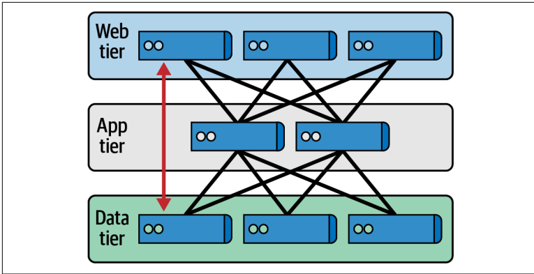
Figure 6-2. An obvious illegal path in the network, and a possible intrusion
