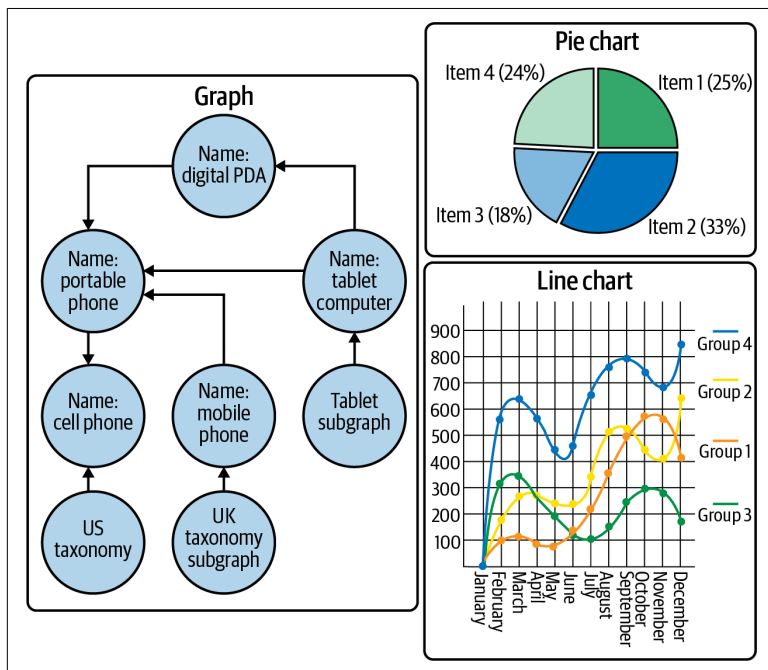
Figure 1-1. Graphs versus charts
