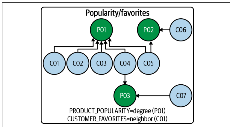
Figure 2-1. A snapshot of customers and their purchases as a plain old graph
