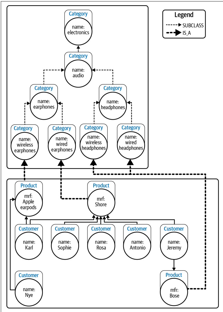
Figure 2-4. A product catalog hierarchy layered on top of the customer and sales data depicted in Figure 2-2
