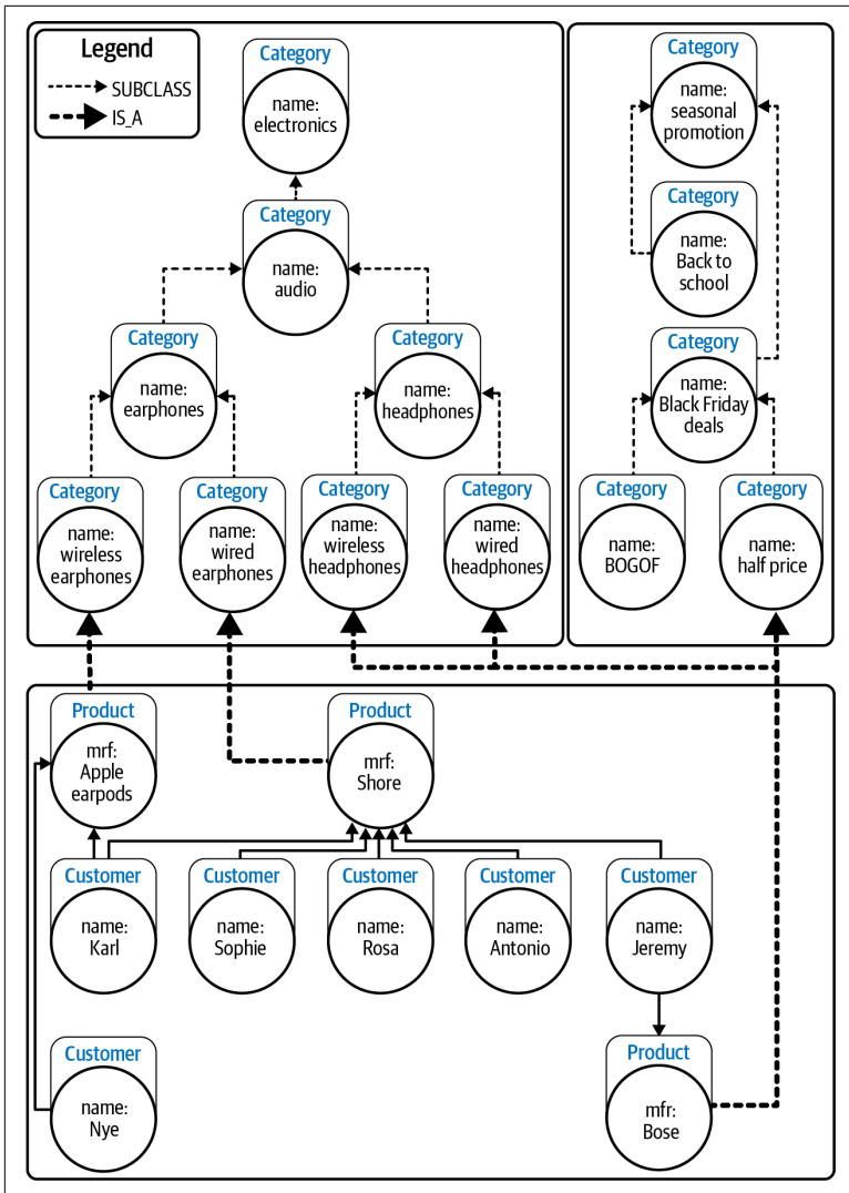
Figure 2-5. Multiple hierarchies can be dynamically layered on top of the customer and sales data; this diagram adds one more level to the contents of Figure 2-4
