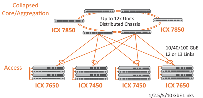
Figure 4: Two-tier campus network.
