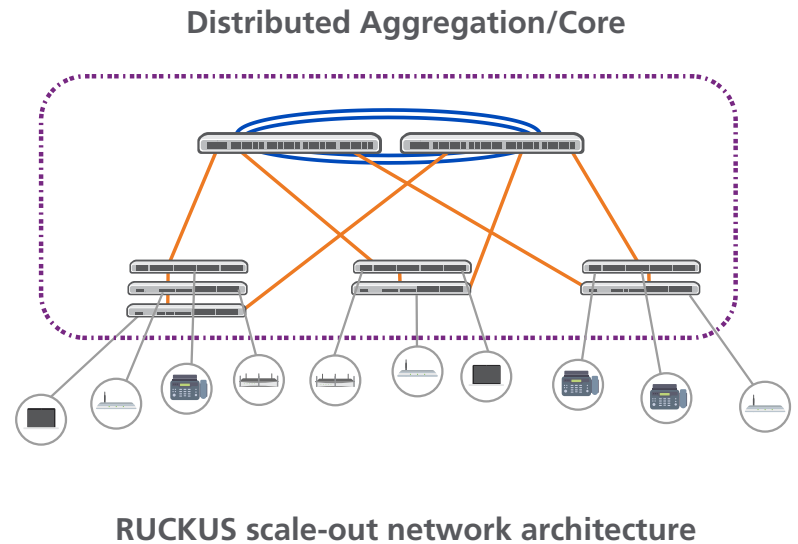
Figure 2: The RUCKUS scale-out architecture versus a traditional multi-tier campus network.
